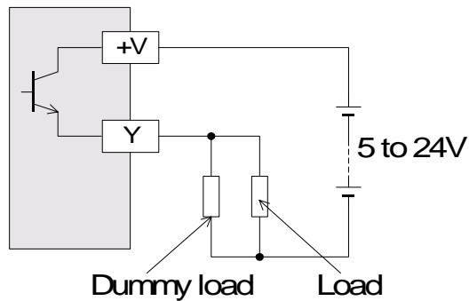
Figure 6.2: Dummy load
