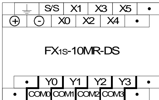
Figure 2.2: Terminal Layouts, Relay Outputs, DC Power
