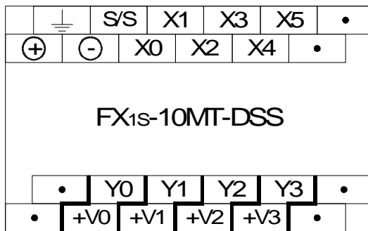
Figure 2.3: Terminal Layouts, Transistor Outputs, DC Power
