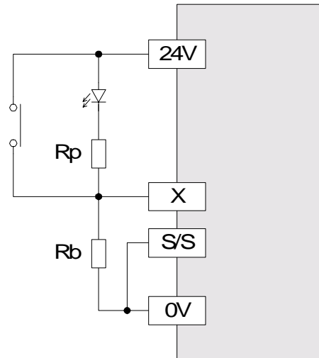
Figure 5.4: Parallel LED Diagram
