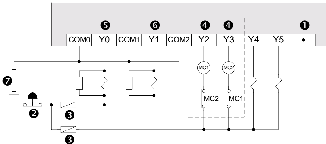
Figure 6.4: Japanese Model Transistor Output
