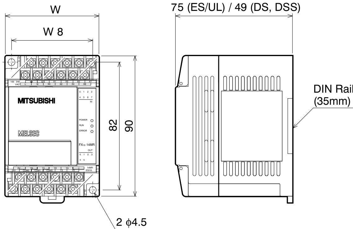
Figure 1.1: FX1s Outline Drawing
