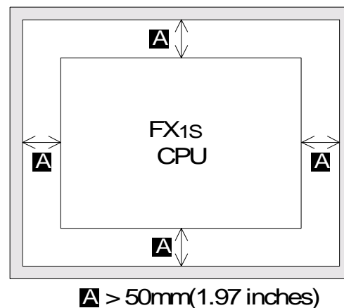
Figure 3.3: PLC Mounting Diagram
