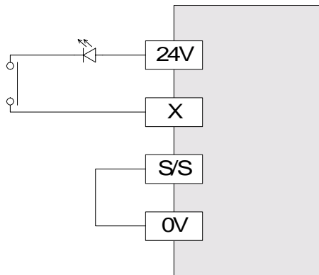
Figure 5.3: Diode Connection Diagram
