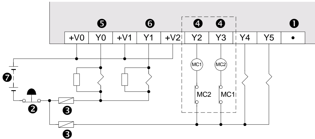
Figure 6.3: Transistor Output Wiring Diagram
